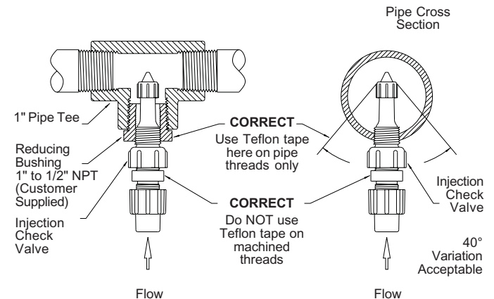
Typical Injection Check Valve Installations
